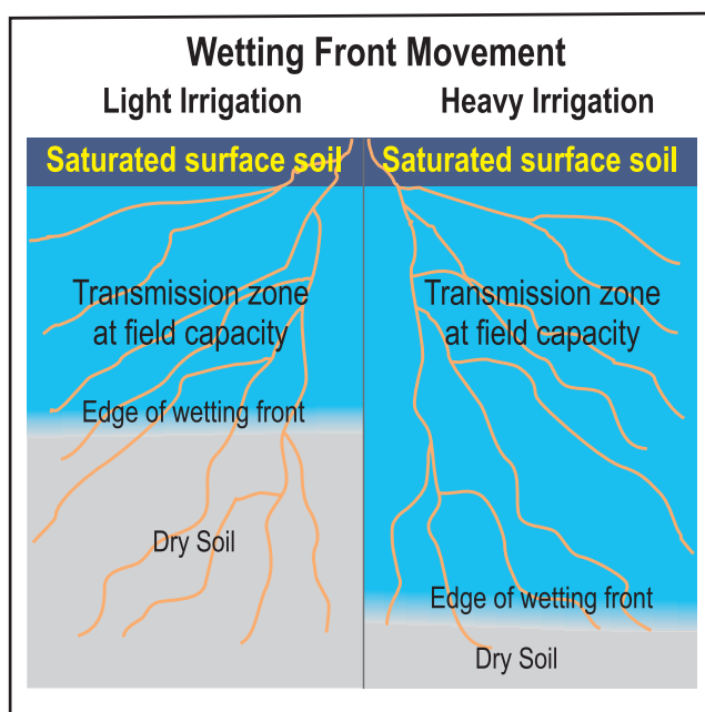
Figure 4: Wetting Front Movement
