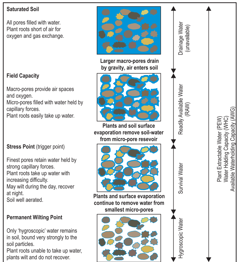
Figure 1: Soil - water storage and movement
