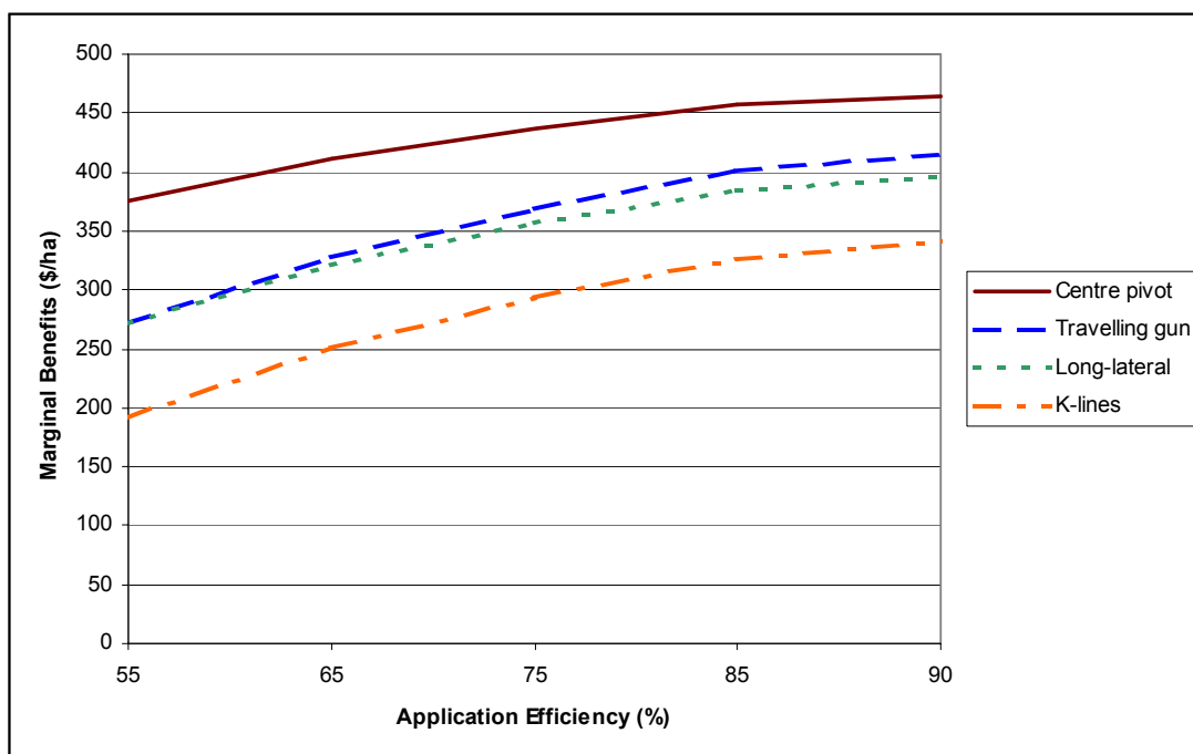
Figure 4: Relationship between application efficiency and marginal benefits
