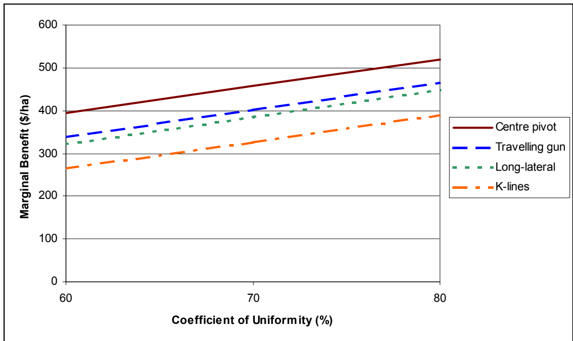
Figure 3: Relationship between application uniformity and marginal benefits
