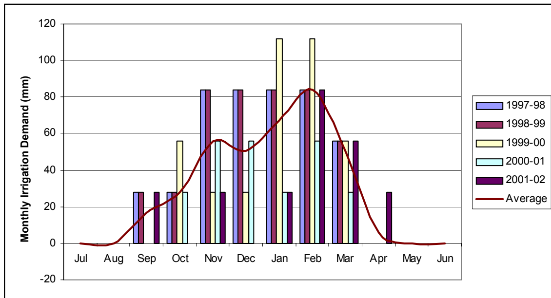
Figure I-1: Irrigation demand at Reporoa (mm/mth) 1998-02
