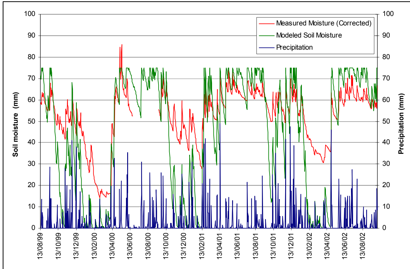
Figure F-1 Comparison of measured and modelled soil moisture levels at Reporoa
