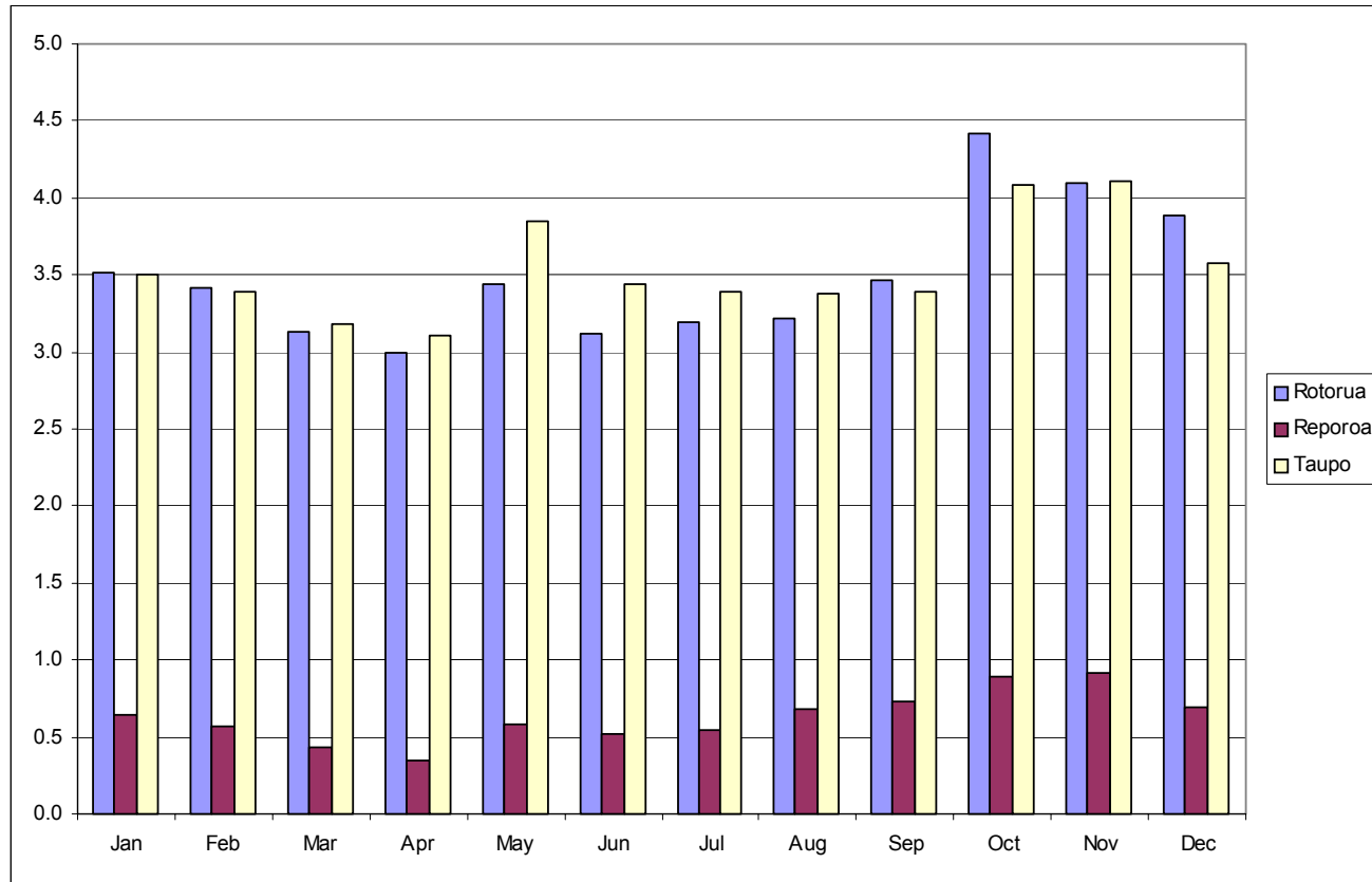
Figure D-1 Comparison of mean monthly wind speed (m/s) for Reporoa, Rotorua and Taupo
