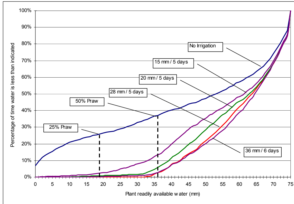
Figure G-1 Plot of soil moisture model levels for non irrigation and irrigation regimes for Reporoa
