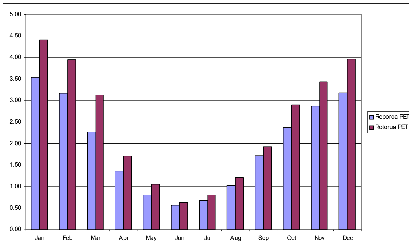
Figure D-1 Comparison of PET (mean monthly (mm/d)) for Reporoa and Rotorua
