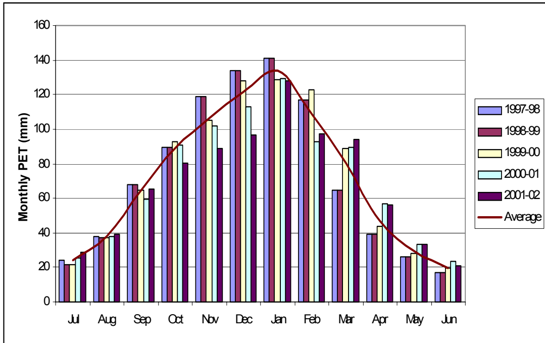
Figure H-2: Monthly PET (mm) at Reporoa
