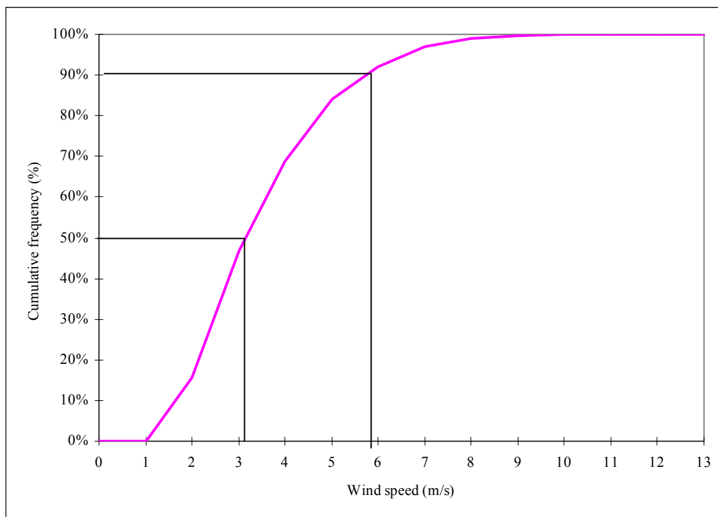
Figure J-1: Cumulative wind speed (%) during irrigation seasons (1998-2002) at Taupo
